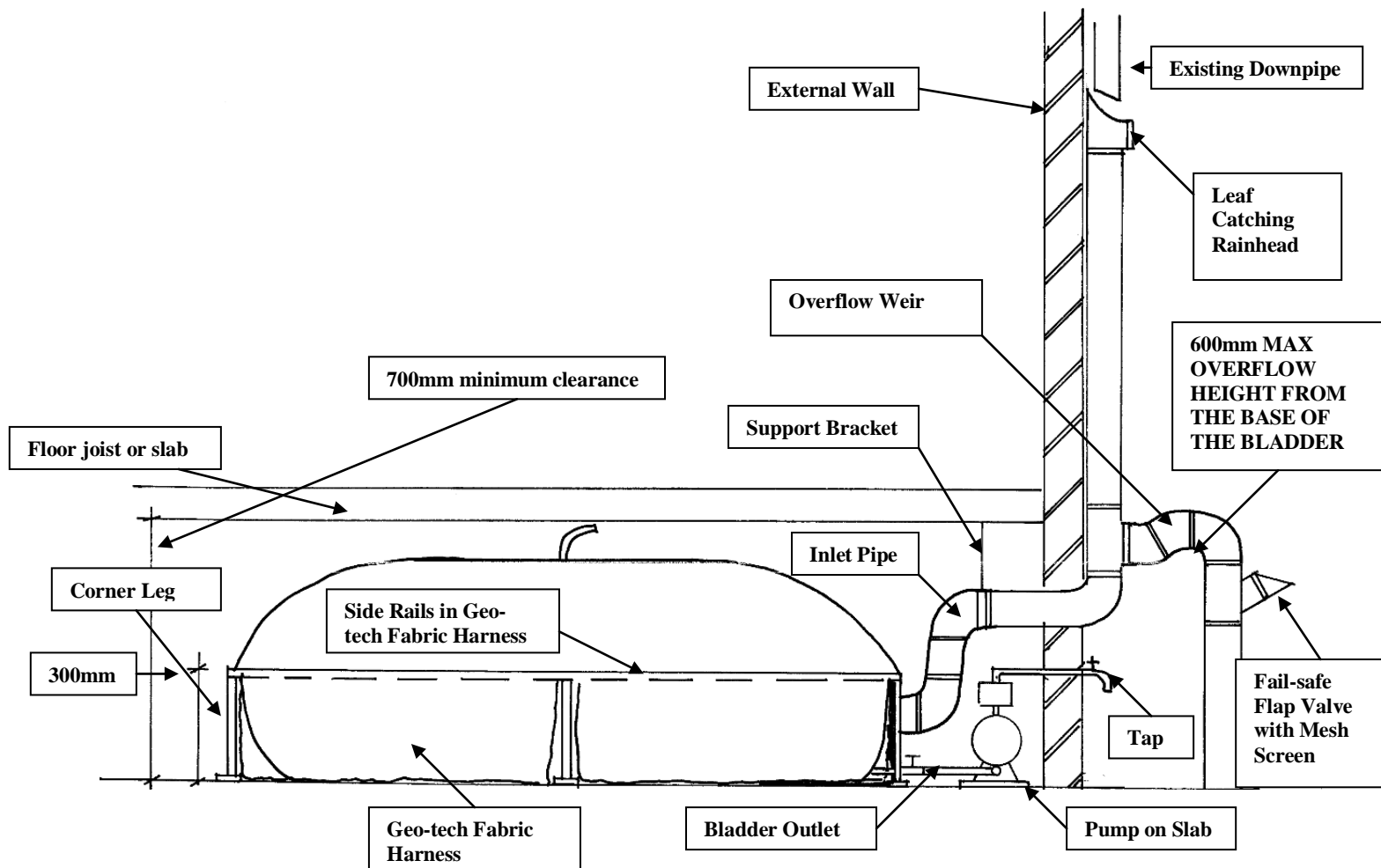
Diagram 5: eco sac® Side View
