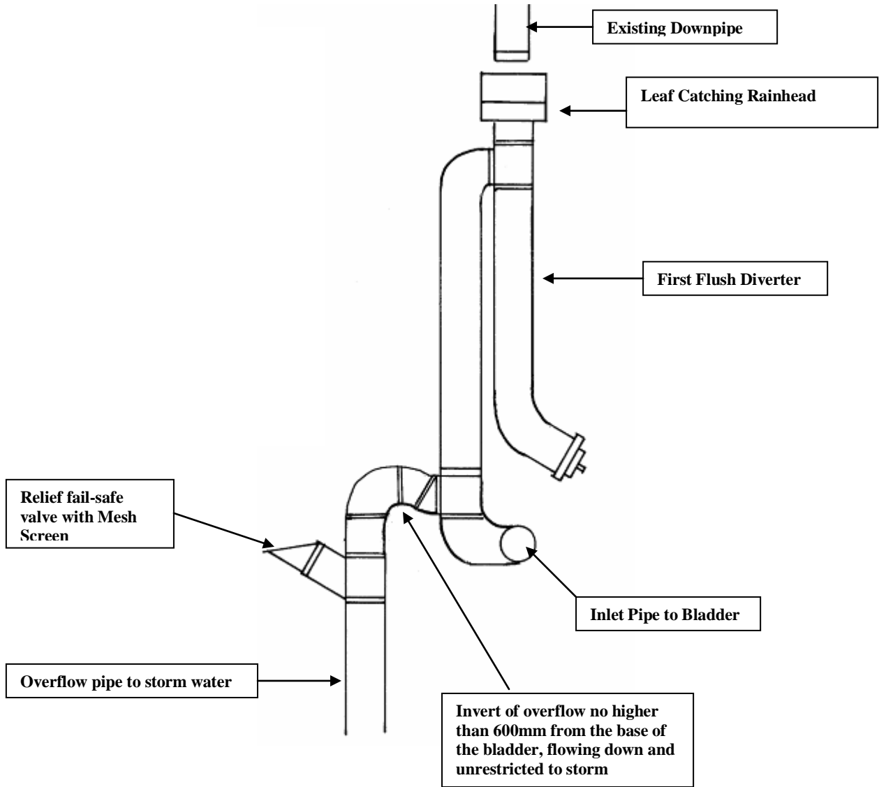
Diagram 1: Down pipe schematic of Inlet with Overflow and Fail Safe Flap Valve
